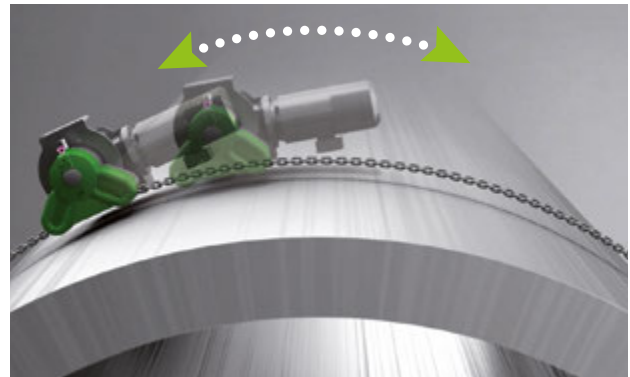
4. Fixed chain, drive / equipment moving along curved path
